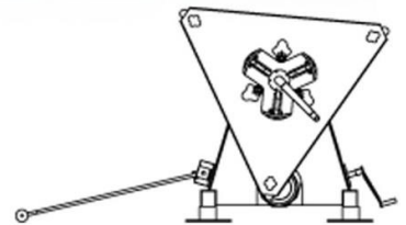
送料架 Uncoiler
